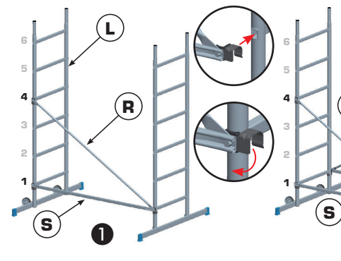
6M DIY ALUMINIUM SCAFFOLD TOWER (4M DIY ALUMINIUM SCAFFOLD TOWER + 2M EXTENSION KIT)
