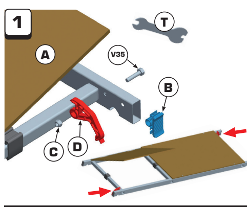
4-5-6-7M DIY ALUMINIUM SCAFFOLD TOWER BASE
